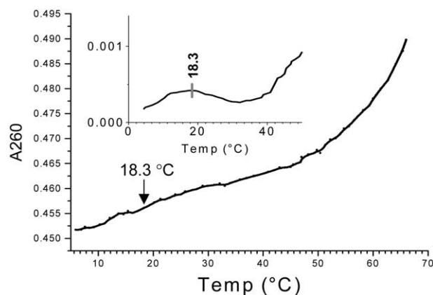
Figure 7. Melting temperature curve for a triple helix containing the 4 -CG base triplet. A T_m value of 18.3 °C was determined from the first derivative of this plot (inset).
