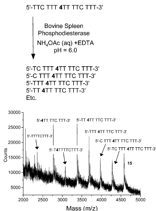
Figure 6. MALDI analysis of an aliquot taken from a bovine spleen phosphodiesterase digestion of oligonucleotide 15 obtained after 24 h.
