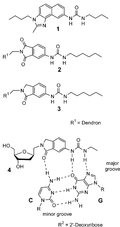
Figure 2. (a) Structures of non-natural receptors designed to form three hydrogen bonds with the major groove side of the CG base pair. (b) Isoindolin-1-one homo- N -nucleoside 4 complexed to CG.
