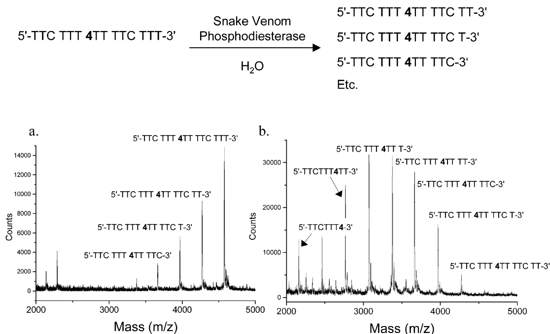
Figure 5. MALDI analysis of digestion of oligonucleotide 15 by snake-venom phosphodiesterase. (a) MALDI spectrum of a digest mixture aliquot after 24 min. (b) MALDI spectrum of a digest mixture aliquot after 290 min.
