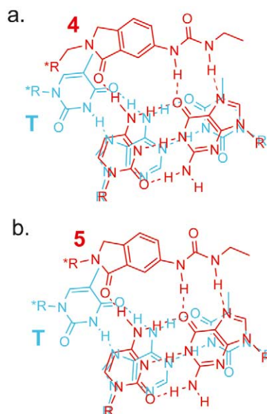
Figure 3. (a) Two-dimensional overlay of the 4 -CG base triplet (red) with the T-AT base triplet (blue). (b) Two-dimensional overlay of the N -nucleoside containing 5 -CG base triplet (red) with the T-AT (blue). (R = 2'-deoxyribose of Watson and Crick strands and *R = 2'-deoxyribose of the TFO.)
