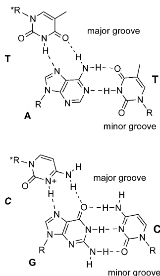
Figure 1. Canonical base triplets in the pyrimidine-purine-pyrimidine (pyr-pur-pyr) triple helix motif. (R = 2'-deoxyribose of Watson and Crick strands and *R = 2'-deoxyribose of the TFO.)
